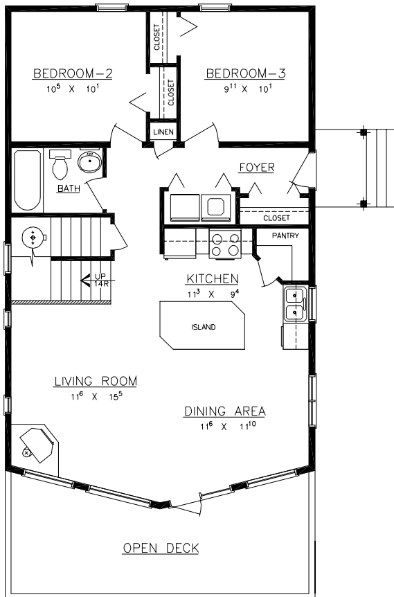
MAIN FLOOR AREA = 900 S.F.
