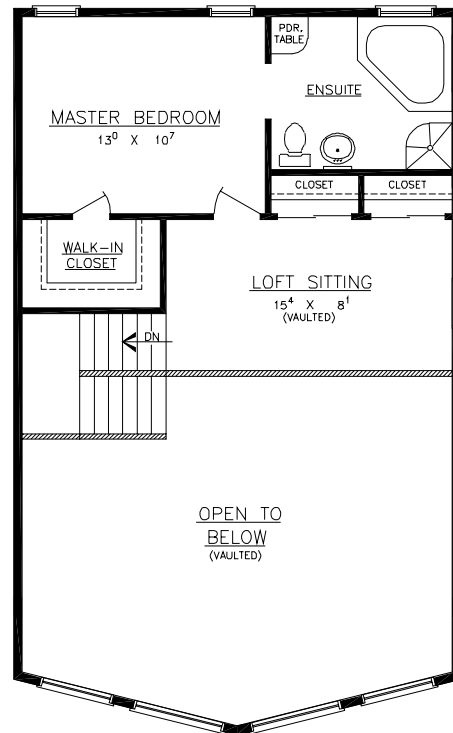
SECOND FLOOR AREA = 446 S.F.
